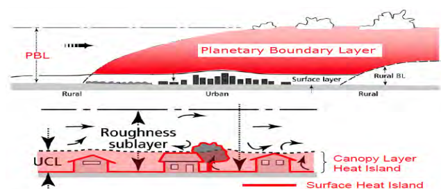
Fig. 2 Types of UHIs and their influence area [11]
